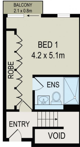
UPPER FLOOR
